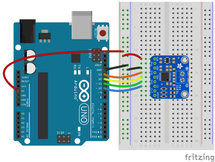
Fritzing diagram.fzz
