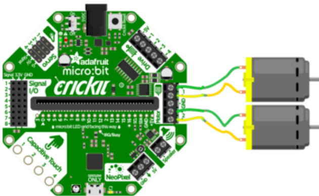
fritzing
