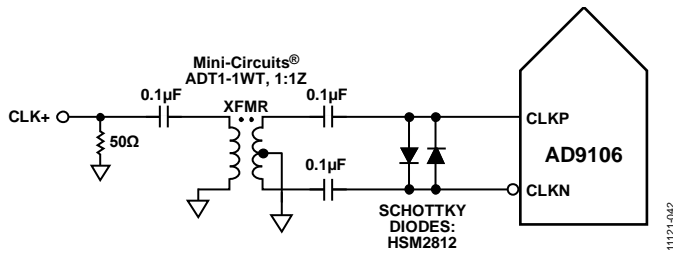
Figure 41. Transformer Coupled Clock
