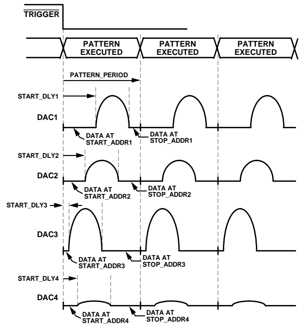
Figure 42. Periodic Pulse Trains Output on All DACs
