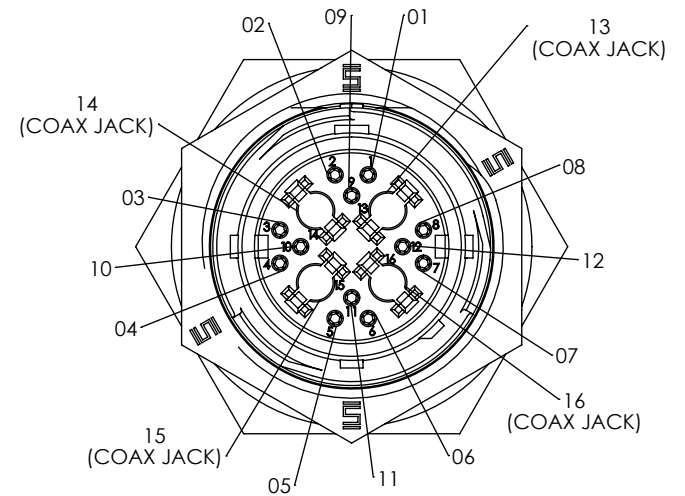
*-06: 16 POS COMBO 4 X COAX JACK 12 X Ø 1.0 SOCKETS
