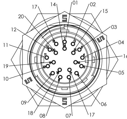
-02: 20 POS Ø 1.0 TERMINALS
