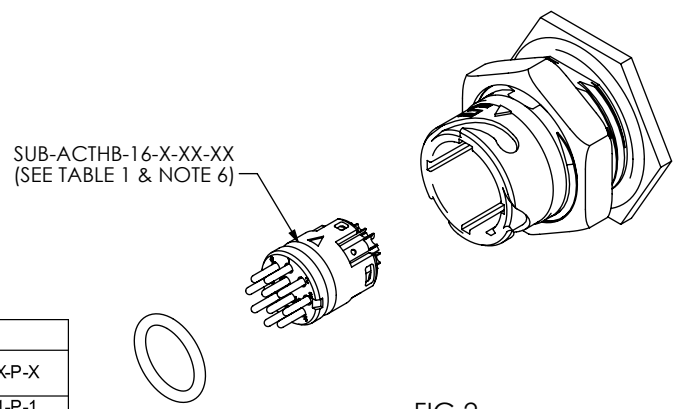
FIG 2 ACRK-16-02-X-T-C-P-1 SHOWN (SAME AS FIG 1, EXCEPT AS SHOWN)
