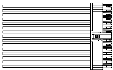
-01: 30 POS (MMSD-15-24-L-XX.XX-S-K)
