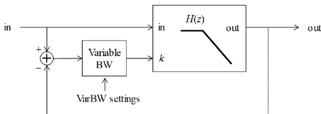
Figure 5: Low-Pass Filter
