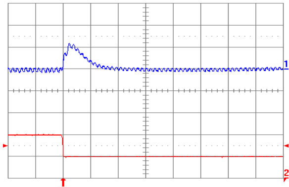
Fig. 2.5V.8: Output voltage response for V_{out} = 2.5\text{ V} to negative load current step change from 10\text{ A} to 5\text{ A} with slew rate of -5\text{ A}/\mu\text{s} at V_{in} = 5\text{ V} . Top trace: output voltage ( 100\text{ mV/div.} ); Bottom trace: load current ( 5\text{ A/div.} ). C_o = 47\text{ }\mu\text{F} ceramic + 1\text{ }\mu\text{F} ceramic. Time scale: 20\text{ }\mu\text{s/div.}
