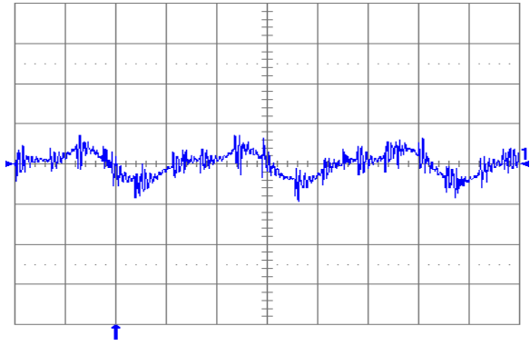
Fig. 2.5V.6: Output voltage ripple ( 20\text{ mV/div.} ) at full rated load current into a resistive load with external capacitance 47\text{ }\mu\text{F} ceramic + 1\text{ }\mu\text{F} ceramic, and V_{in} = 5\text{ V} for V_{out} = 2.5\text{ V} . Time scale: 2\text{ }\mu\text{s/div.}
