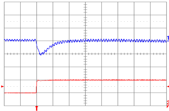
Fig. 2.5V.7: Output voltage response for V_{out} = 2.5\text{ V} to positive load current step change from 5\text{ A} to 10\text{ A} with slew rate of 5\text{ A}/\mu\text{s} at V_{in} = 5\text{ V} . Top trace: output voltage ( 100\text{ mV/div.} ); Bottom trace: load current ( 5\text{ A/div.} ). C_o = 47\text{ }\mu\text{F} ceramic + 1\text{ }\mu\text{F} ceramic. Time scale: 20\text{ }\mu\text{s/div.}
