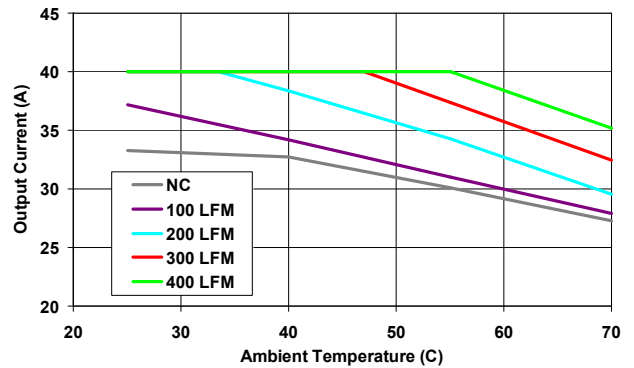
Figure 13. Output Current Derating at V_o=1.2Vdc
