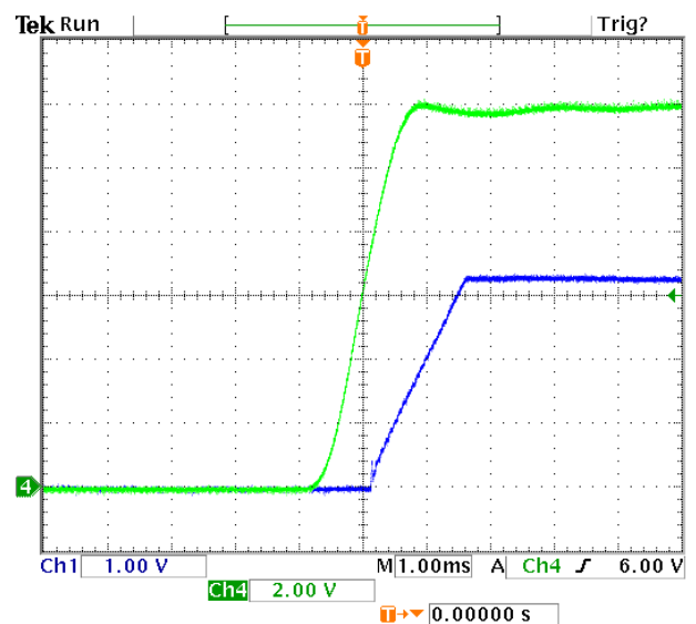
Figure 8. Typical Start-Up with application of Vin (Vo = 3.3Vdc, Io = 40A). Ch1 – Vout, Ch2 – Vin
