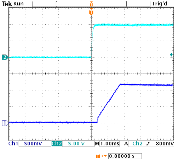
Figure 5. Typical Start-Up Using Remote On/Off (Vo = 1.2Vdc, Io=40A). Ch1 – Vout, Ch2 – ON/OFF
