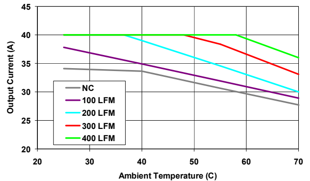
Figure 12. Output Current Derating at V_o=0.6Vdc
