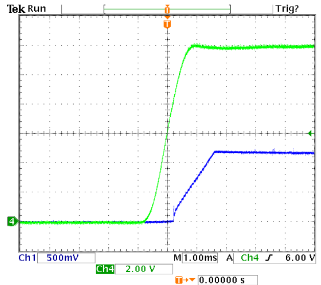
Figure 7. Typical Start-Up with application of Vin (Vo = 1.2Vdc, Io = 40A). Ch1 – Vout, Ch2 – Vin
