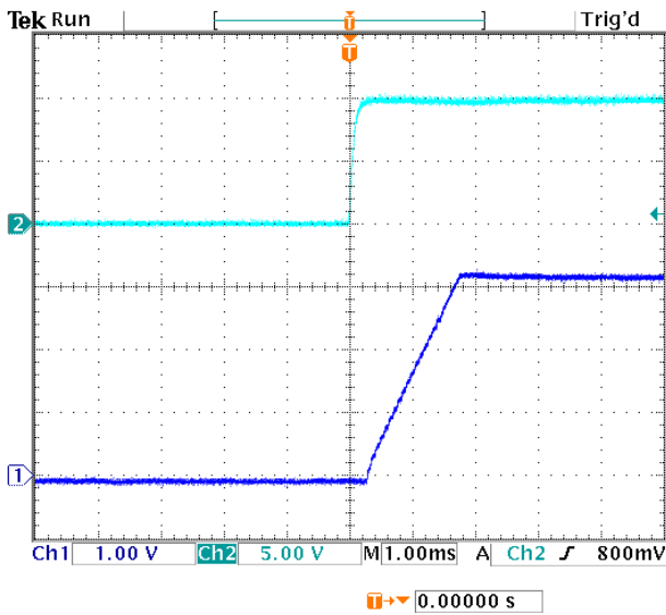
Figure 6. Typical Start-Up Using Remote On/Off (Vo = 3.3Vdc, Io=40A). Ch1 – Vout, Ch2 – ON/OFF
