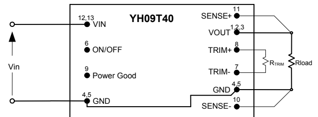
Figure 17. Programming Output Voltage With A Resistor
