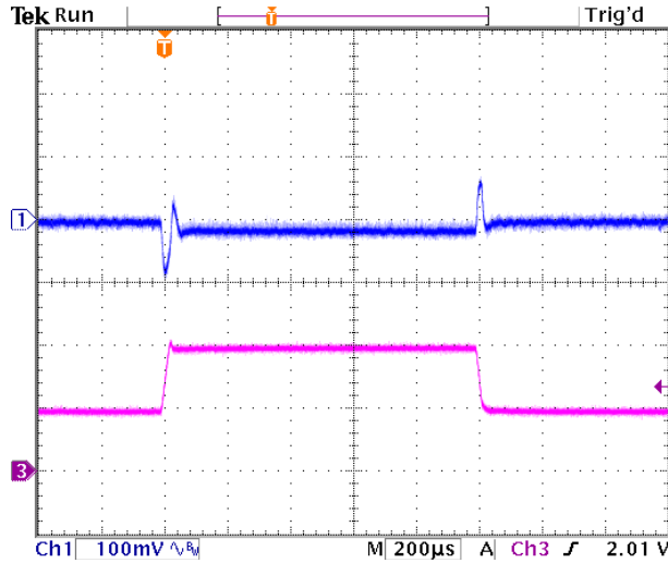
Figure 9. Transient Response to Dynamic Load Change from 50% to 100% of full load ( V_{in}=12V , V_o=0.6Vdc ). Ch3 – iout. Scale=20A/div
