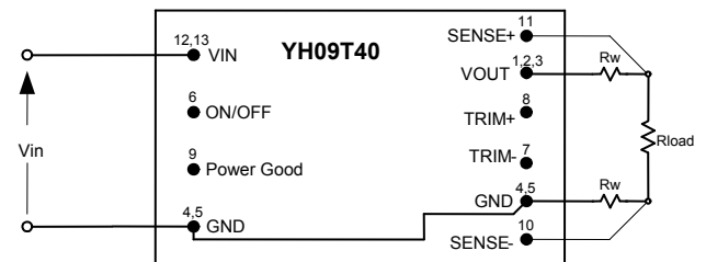
Figure 19. Remote Sense Circuit Configuration
