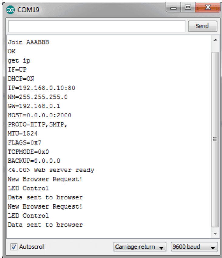
Arduino serial comm output when an HTTP request is sent to the shield.
