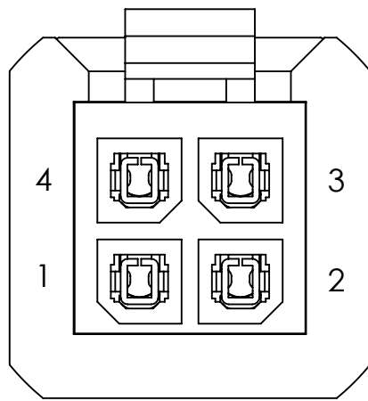
Connector pin-out View into Router (rear view of cable connector)
