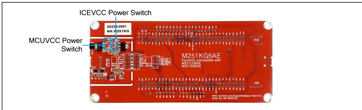
Figure 3-2 Rear View of NuMaker-M251KG
