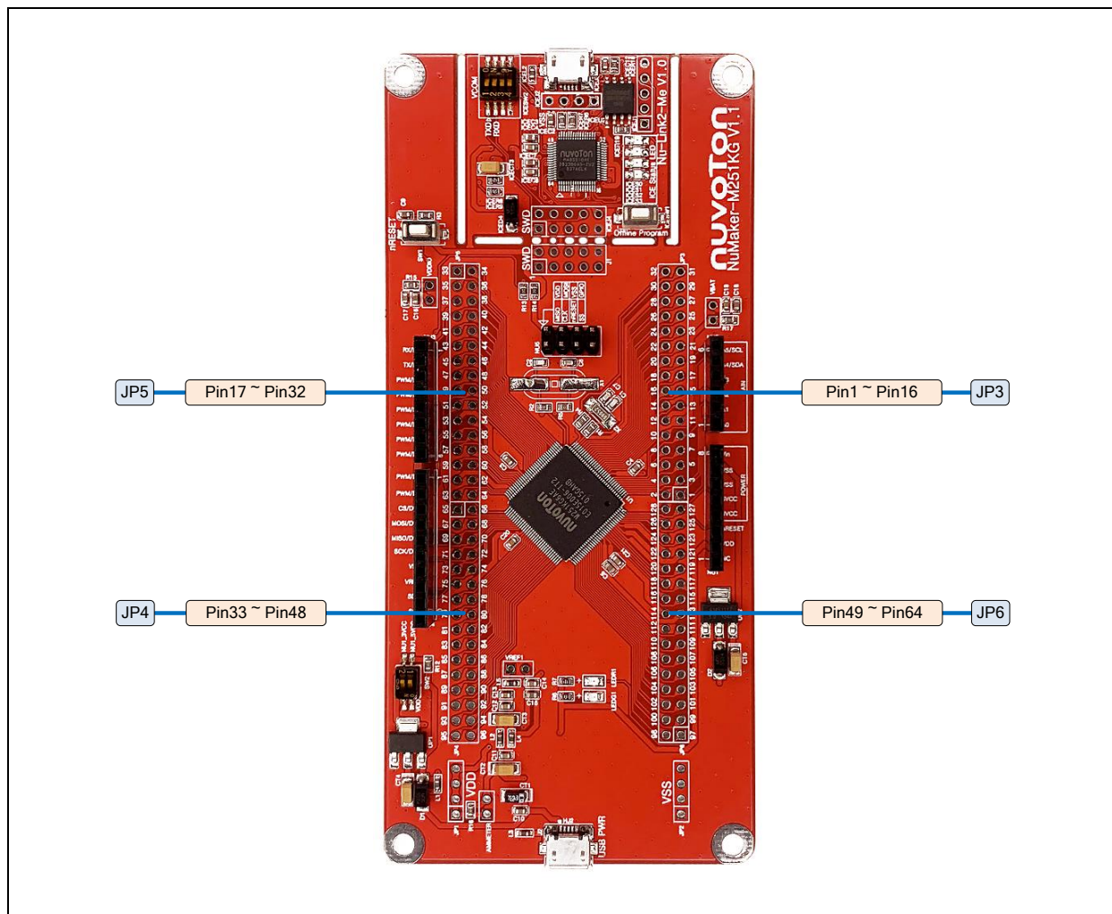
Figure 3-3 M251KG6AE Extension Connectors
