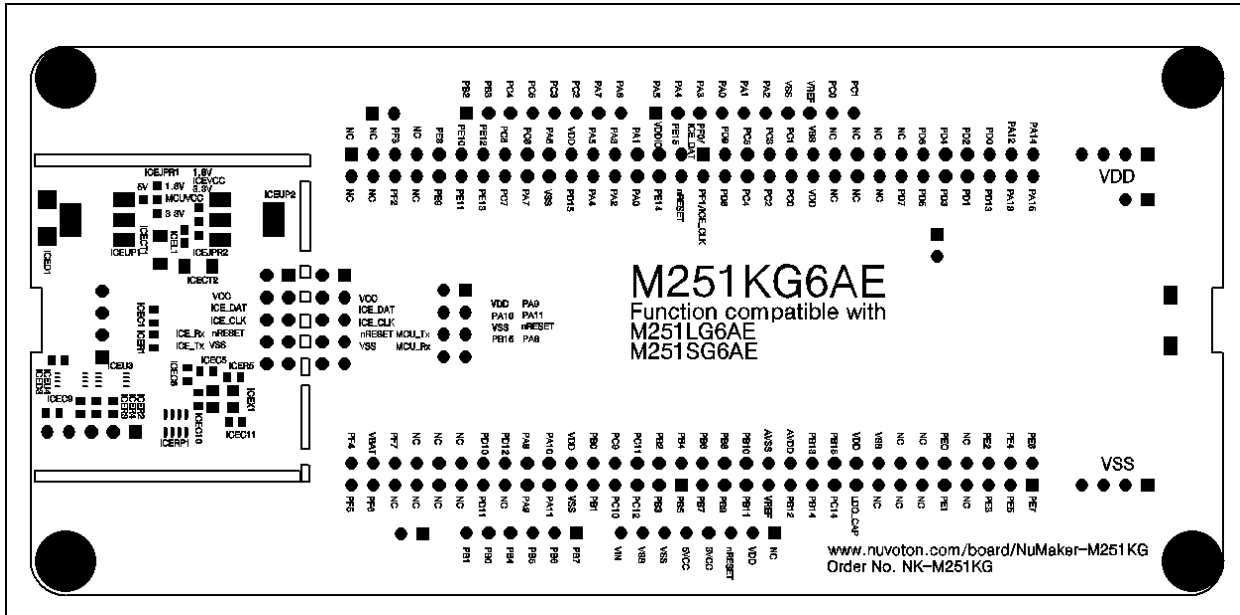
Figure 5-5 Rear Placement
