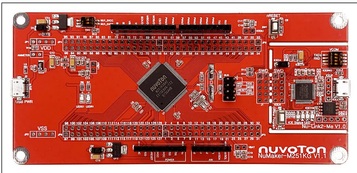
Figure 1-1 NuMaker-M251KG Board
