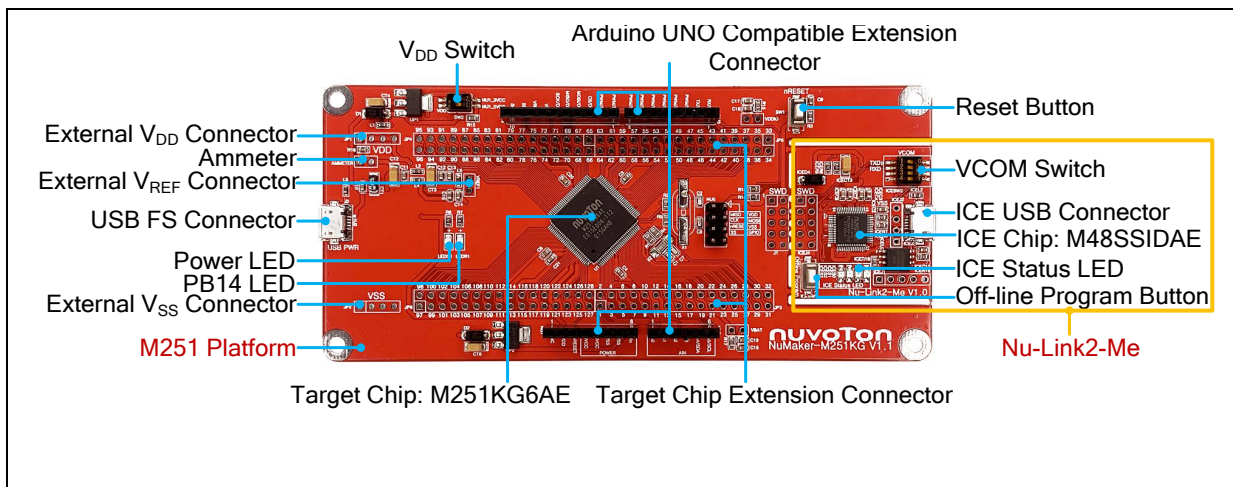
Figure 3-1 Front View of NuMaker-M251KG
