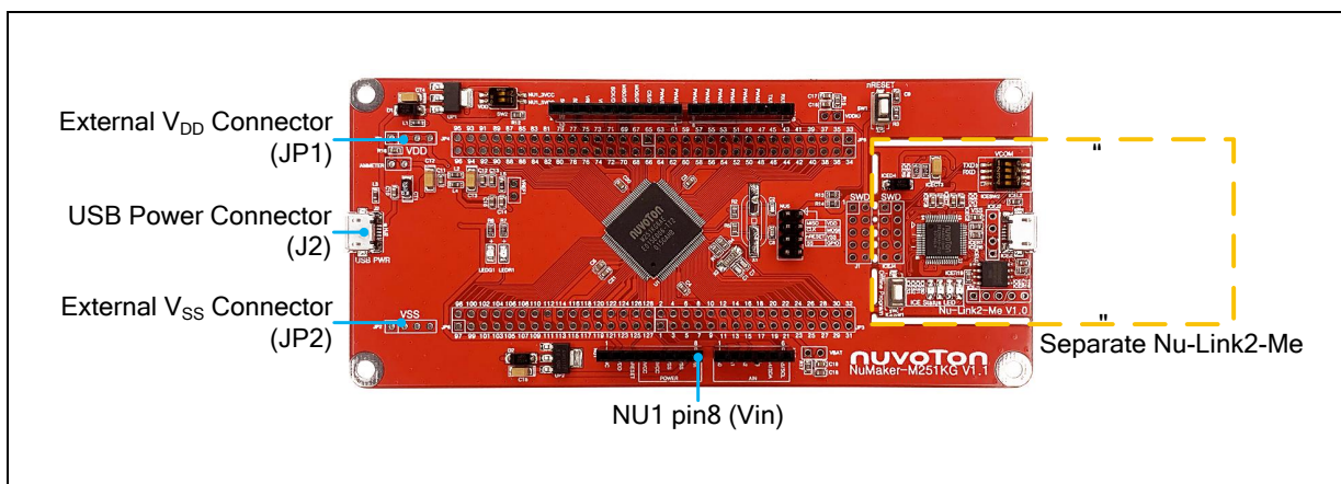
Figure 3-7 Separate the Nu-Link2-Me from NuMaker-M251KG
