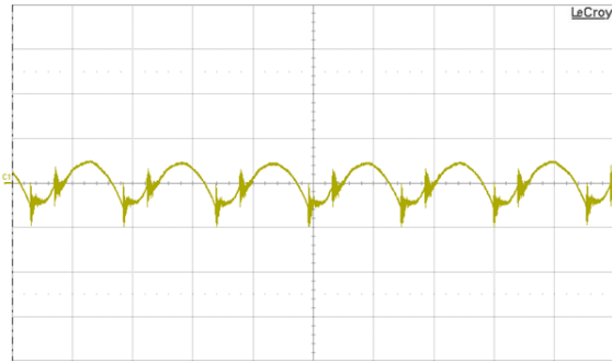
Fig. 13: Output voltage ripple (50 mV/div.) at full rated load current into a resistive load with C_o = 10 \mu\text{F} tantalum + 1 \mu\text{F} ceramic and V_{in} = 48 \text{ V} . Time scale: 1 \mu\text{s}/\text{div} .
