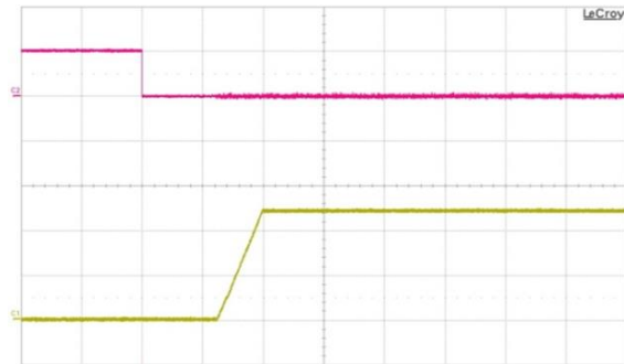
Fig. 12: Output voltage response to load current step-change (3A – 4.5A – 3A) at V_{in} = 48 \text{ V} . Current slew rate: 0.1 \text{ A}/\mu\text{s} . C_o = 270\mu\text{F} E-cap + 1 \mu\text{F} ceramic + 10 \mu\text{F} tantalum. Time scale: 500 \mu\text{s}/\text{div} .
