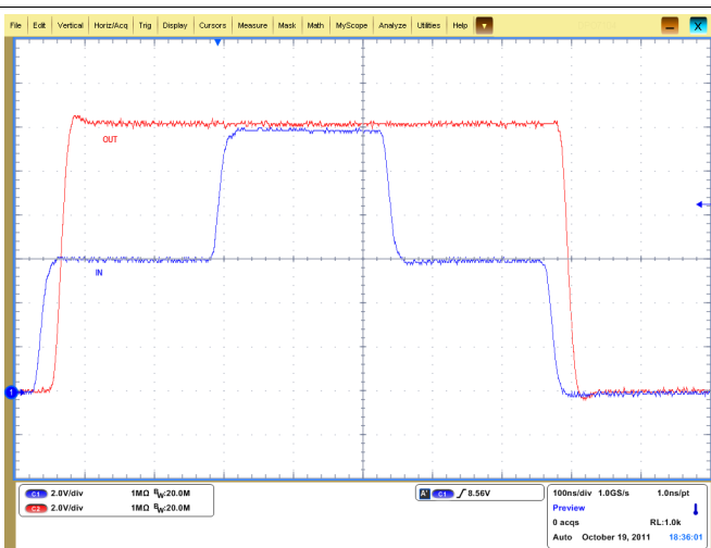
Figure 36. Step Input
