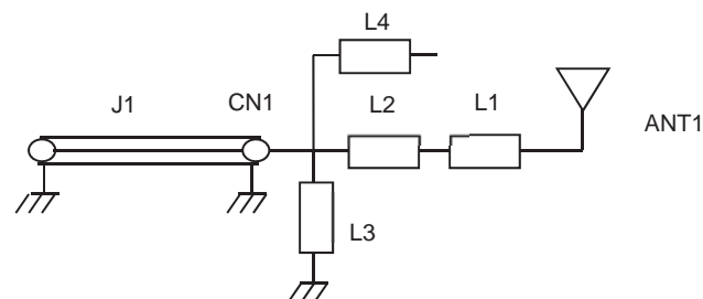
Fig. 2. Equivalent circuit
