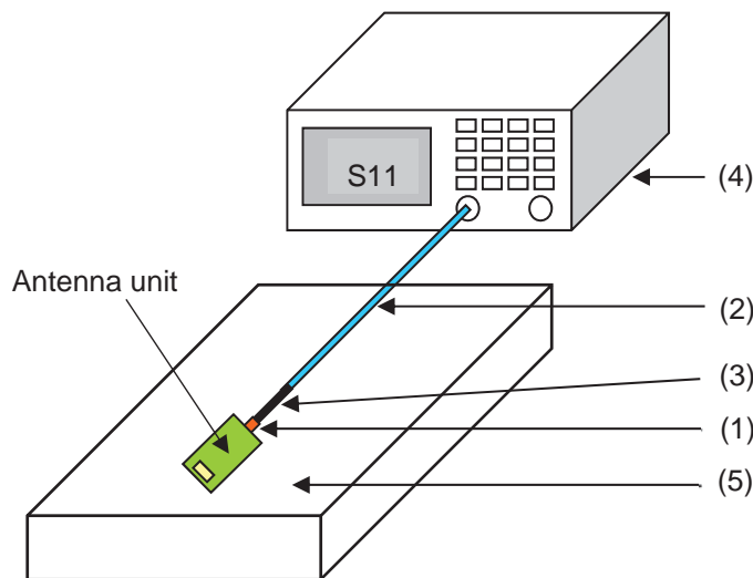
Fig. 3. Method of measuring VSWR
