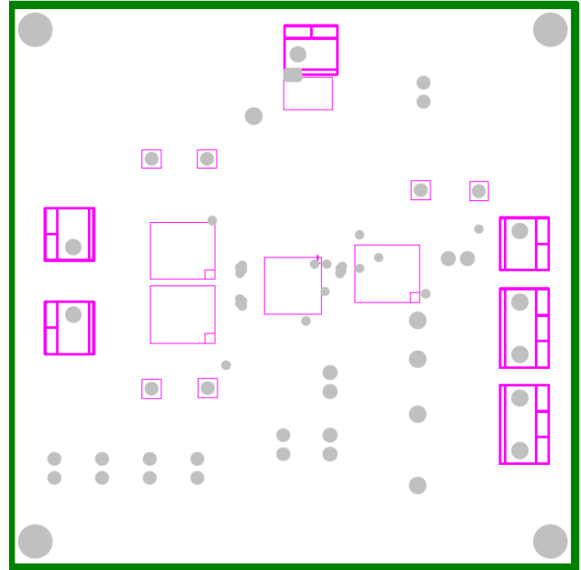
Figure 4. Board Layout (Middle 2 nd ) Layer
