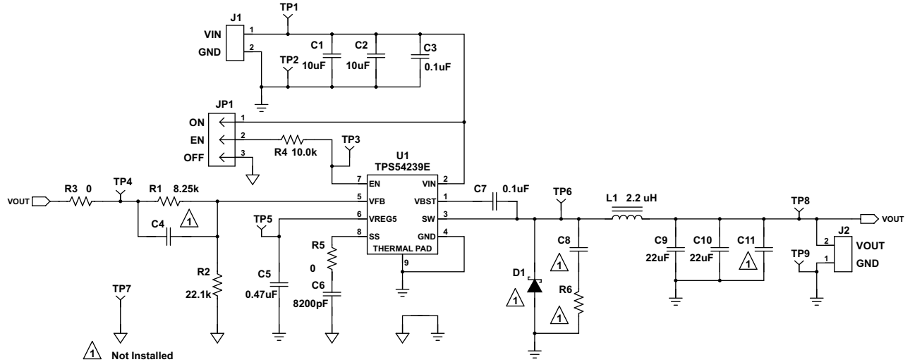
Figure 19. TPS54239EVM-056 Schematic Diagram
