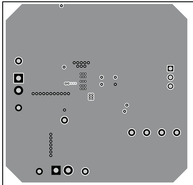
Figure 17. Internal Layer 2
