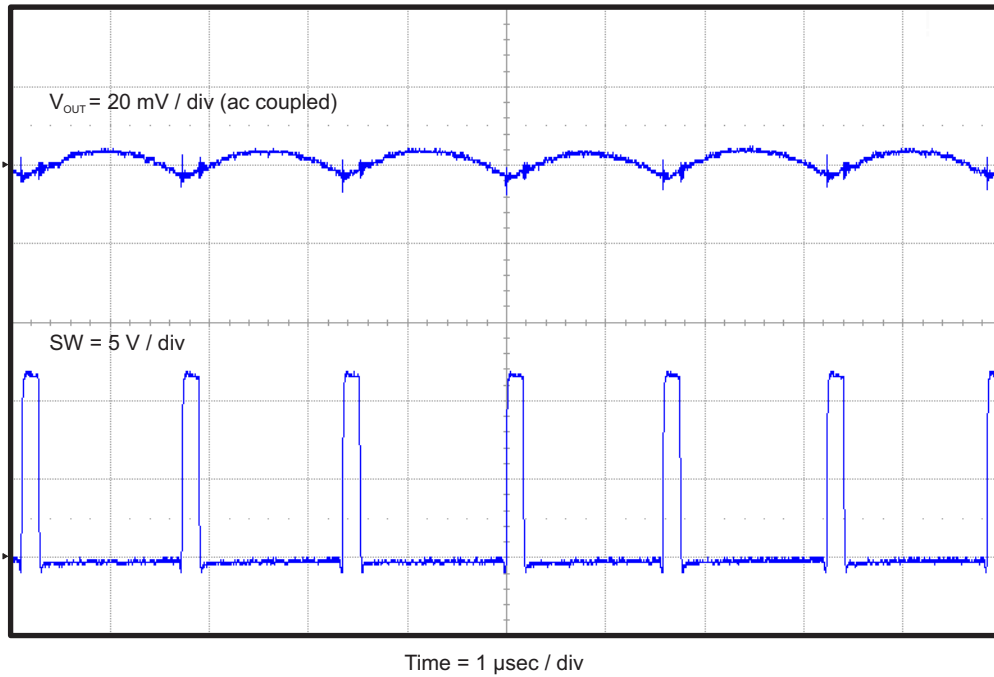
Figure 6. TPS54239EEVM-056 Output Voltage Ripple ( I_{OUT} = 2 \text{ A} )
