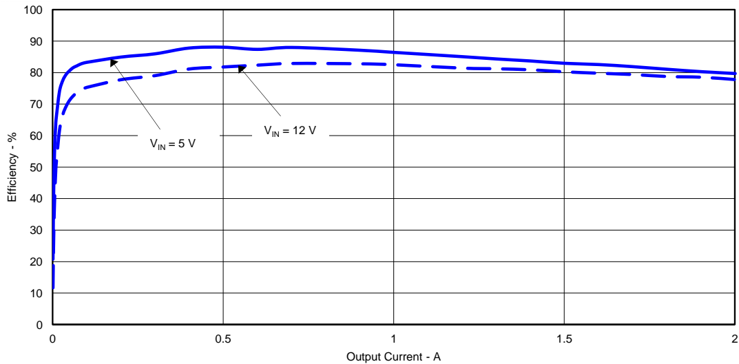
Figure 1. TPS54239EEVM-056 Efficiency
