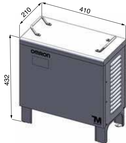
Control Box
