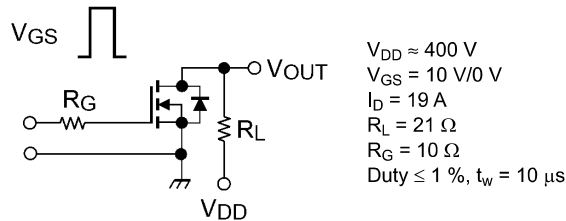
Fig. 6.2.1 Switching Time Test Circuit
