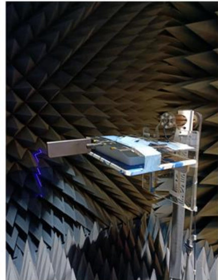
30x30cm Ground plane (Edge)
