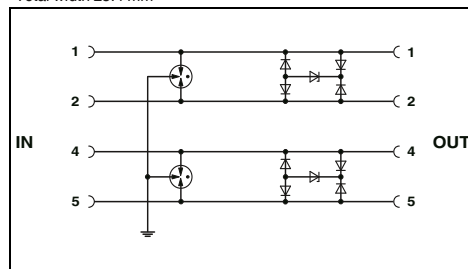
Total width 25.4 mm
