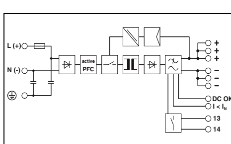
Power supply, dip-coated, 1 AC, 24 V DC, 5 A
