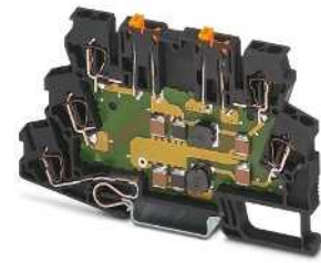
Protection for two conductors with a common reference potential
