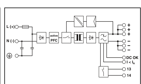
Power supply, dip-coated, 1 AC, 24 V DC, 10 A
