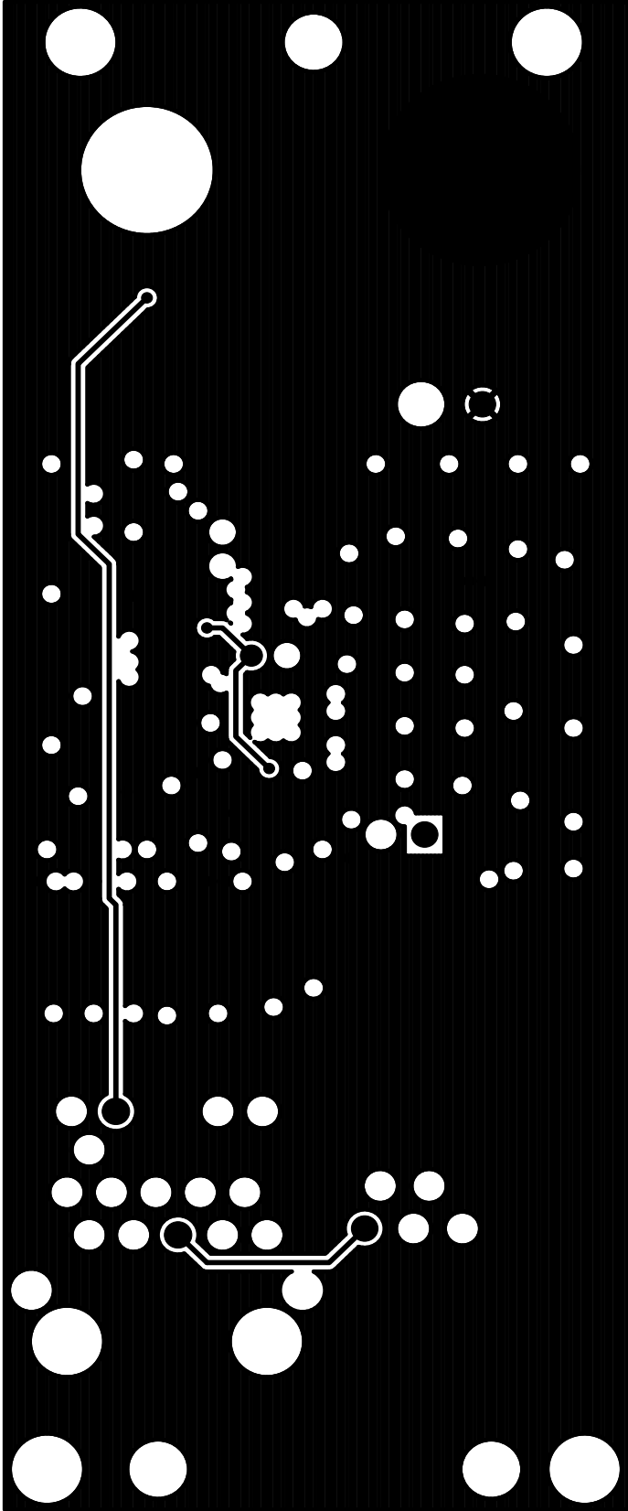
Figure 5. Internal 2 (Layer 3)
