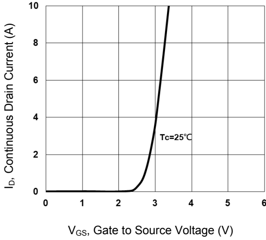
Figure 7. Transfer Characteristics
