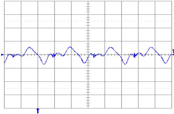
Fig. 1.5V.7: Output voltage ripple (20 mV/div.) at full rated load current into a resistive load with C_o = 10 \mu\text{F} tantalum + 1 uF ceramic and V_{in} = 48 \text{ V} . Time scale: 1 \mu\text{s}/\text{div} .
