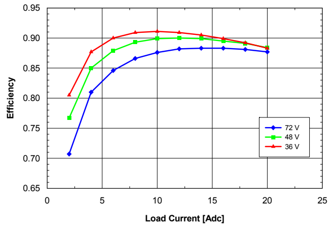
Fig. 2.5V.2: Efficiency vs. load current and input voltage for SQM48T/S20025 converter mounted vertically with air flowing from pin 3 to pin 1 at a rate of 300 LFM (1.5 m/s) and T_a = 25\text{ }^\circ\text{C} .
