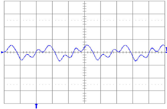
Fig. 2.0V.7: Output voltage ripple (20 mV/div.) at full rated load current into a resistive load with C_o = 10 \mu\text{F} tantalum + 1 uF ceramic and V_{in} = 48 \text{ V} . Time scale: 1 \mu\text{s}/\text{div} .
