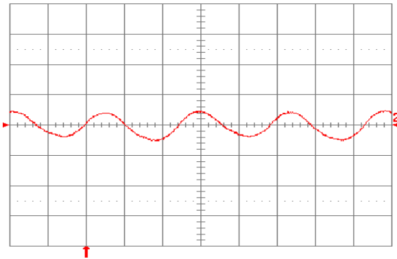
Fig. 3.3V.9: Input reflected ripple current, i_c (100 mA/div.), measured at input terminals at full rated load current and V_{in} = 48 \text{ V} . Refer to Fig. 3.3V.8 for test setup. Time scale: 1 \mu\text{s}/\text{div} .
