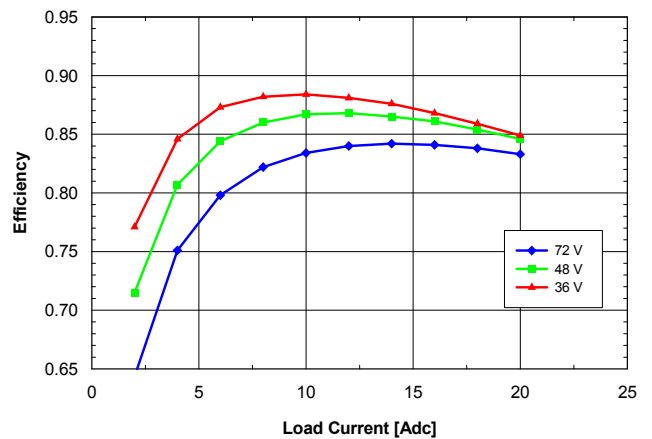
Fig. 1.5V.2: Efficiency vs. load current and input voltage for SQM48T/S20015 converter mounted vertically with air flowing from pin 3 to pin 1 at a rate of 300 LFM (1.5 m/s) and T_a = 25\text{ }^\circ\text{C} .
