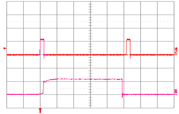
Fig. 1.8V.12: Load current (top trace, 20 A/div., 20 ms/div.) into a 10 mΩ short circuit during restart, at V in = 48 V. Bottom trace (20 A/div., 1 ms/div.) is an expansion of the on-time portion of the top trace.
