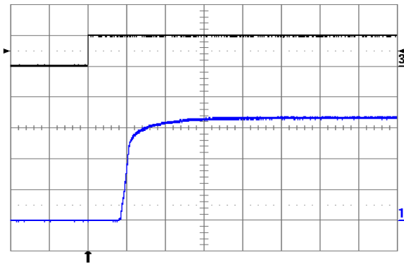
Fig. 3.3V.3: Turn-on transient at full rated load current (resistive) with no output capacitor at V_{in} = 48\text{ V} , triggered via ON/OFF pin. Top trace: ON/OFF signal (5V/div.). Bottom trace: output voltage (1 V/div.). Time scale: 2 ms/div.
