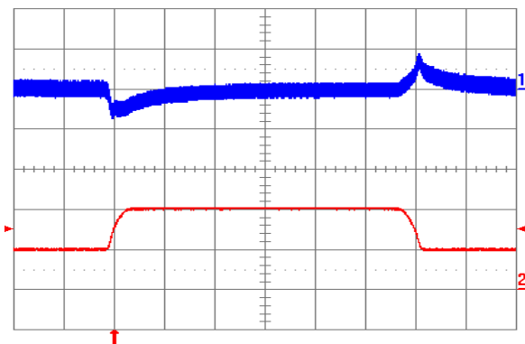
Fig. 3.3V.5: Output voltage response to load current step-change (5A – 10A – 5A ) at V_{in} = 48\text{ V} . Top trace: output voltage (100 mV/div.). Bottom trace: load current (5A/div.). Current slew rate: 0.1 A/ \mu\text{s} . C_o = 1\ \mu\text{F} ceramic. Time scale: 0.2 ms/div.
