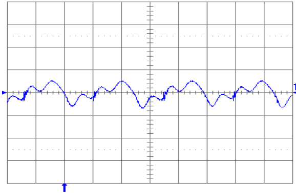
Fig. 1.8V.7: Output voltage ripple (20mV/div.) at full rated load current into a resistive load with C_o = 10 \mu\text{F} tantalum + 1 uF ceramic and V_{in} = 48 \text{ V} . Time scale: 1 \mu\text{s}/\text{div} .
