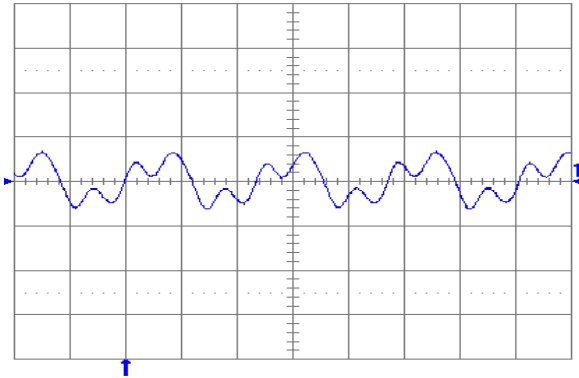
Fig. 2.5V.7: Output voltage ripple (20 mV/div.) at full rated load current into a resistive load with C_o = 10 \mu\text{F} tantalum + 1uF ceramic and V_{in} = 48 \text{ V} . Time scale: 1 \mu\text{s}/\text{div} .
