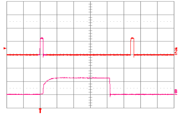
Fig. 1.2V.16: Load current (top trace, 20 A/div., 50 ms/div.) into a 10 mΩ short circuit during restart, at V in = 48 V. Bottom trace (20 A/div., 5 ms/div.) is an expansion of the on-time portion of the top trace.
