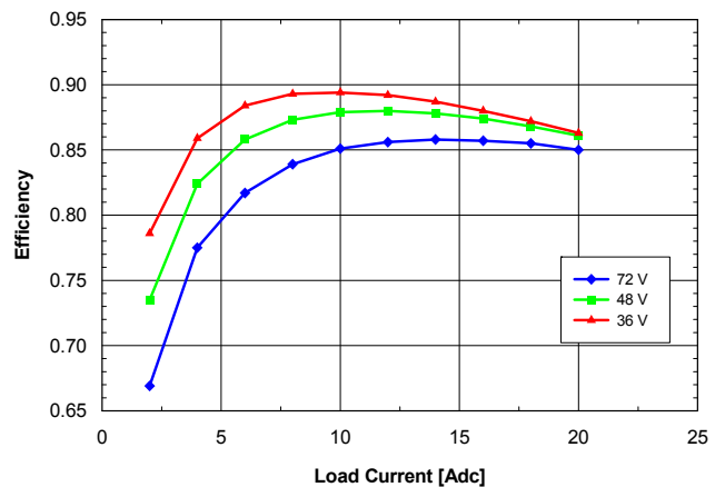
Fig. 1.8V.2: Efficiency vs. load current and input voltage for SQM48T/S20018 converter mounted vertically with air flowing from pin 3 to pin 1 at a rate of 300 LFM (1.5 m/s) and T_a = 25\text{ }^\circ\text{C} .
