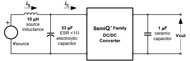
Fig. 1.5V.8: Test setup for measuring input reflected ripple currents, i_c and i_s .
