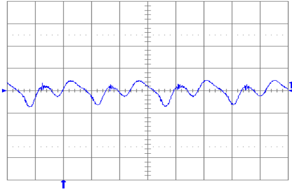
Fig. 1.2V.7: Output voltage ripple (20 mV/div.) at full rated load current into a resistive load with C_o = 10 \mu\text{F} tantalum + 1 uF ceramic and V_{in} = 48 \text{ V} . Time scale: 1 \mu\text{s}/\text{div} .
