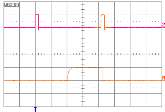
Figure 15. Load current (top trace, 50 A/div., 50 ms/div.) into a 10 m\Omega short circuit during restart, at V_{in} = 48 V. Bottom trace (50 A/div., 5 ms/div.) is an expansion of the on-time portion of the top trace.
