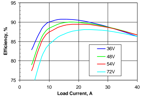
Figure 2. Efficiency vs. load current and input voltage for SQE48T40015 converter mounted vertically with air flowing from pin 3 to pin 1 at 300 LFM (1.5 m/s) and T_a=25\text{ }^\circ\text{C} .
