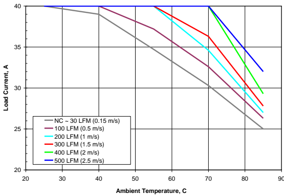
Figure 1. Available load current vs. ambient air temperature and airflow rates for SQE48T40015 converter mounted vertically with air flowing from pin 3 to pin 1, MOSFET temperature \leq 120\text{ }^\circ\text{C} , V_{in} = 48\text{ V} . Note: NC – Natural convection
