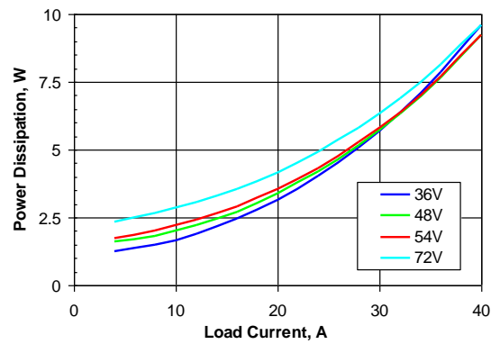
Figure 4. Power dissipation vs. load current and input voltage for SQE48T40015 converter mounted vertically with air flowing from pin 3 to pin 1 at a rate of 300 LFM (1.5 m/s) and T_a = 25\text{ }^\circ\text{C} .
