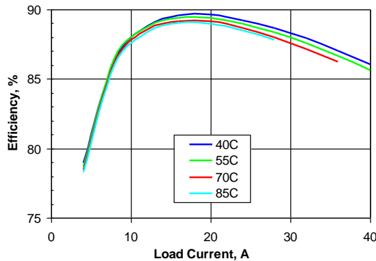
Figure 3. Efficiency vs. load current and ambient temperature for SQE48T40015 converter mounted vertically with V_{in}=48\text{ V} and air flowing from pin 3 to pin 1 at 200LFM (1.0m/s).
