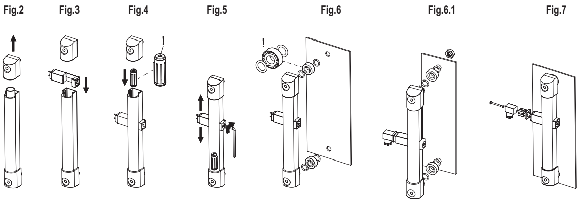
Sensor holder bracket
