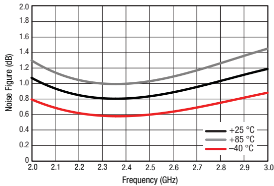
Figure 11. Noise Figure vs Frequency Over Temperature
