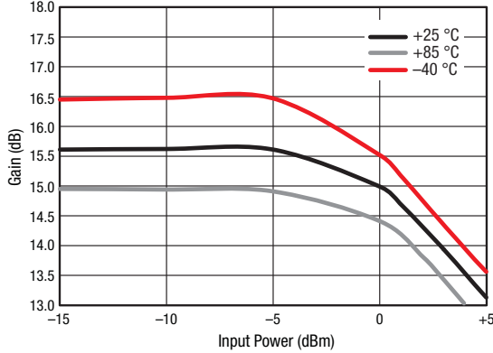
Figure 22. Gain vs Input Power Over Temperature @ 3000 MHz
