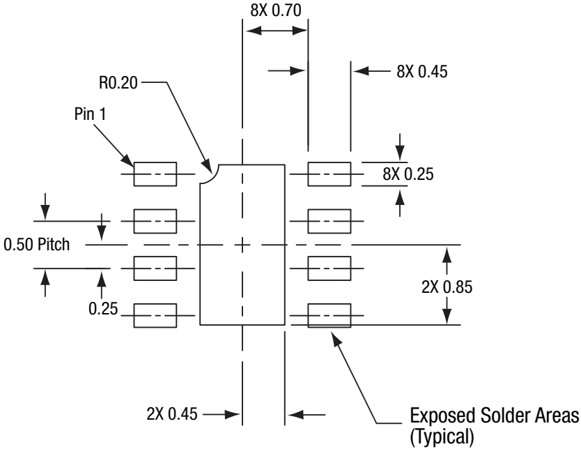
Figure 29. SKY67023-396LF PCB Layout Footprint (Top View)
