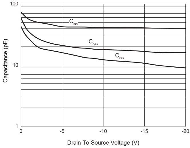
Fig. 7 - Capacitance Characteristics
