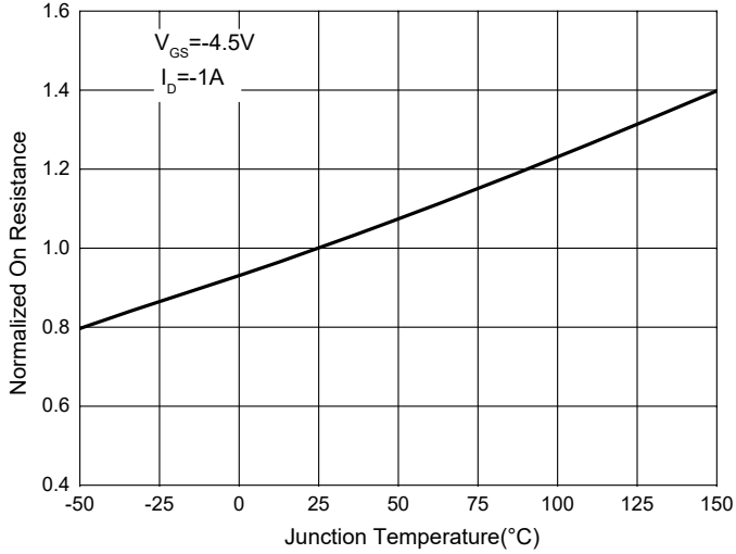
Fig.9-NormalizedOnResistanceCharacteristics
