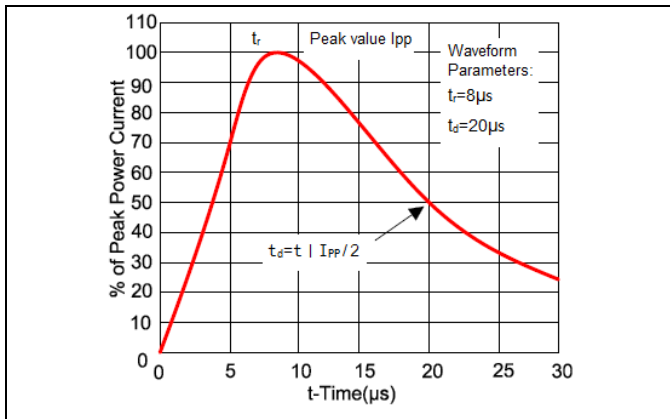
Figure 1. Pulse Waveforms
