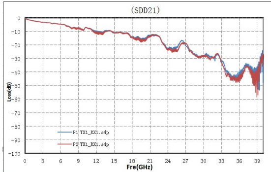
SFP28 30AWG 1M
