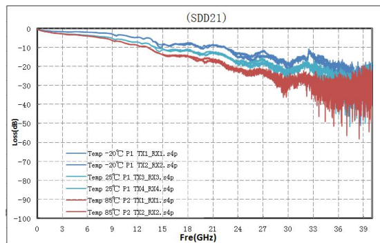
Temperature test data (26AWG 3M)
