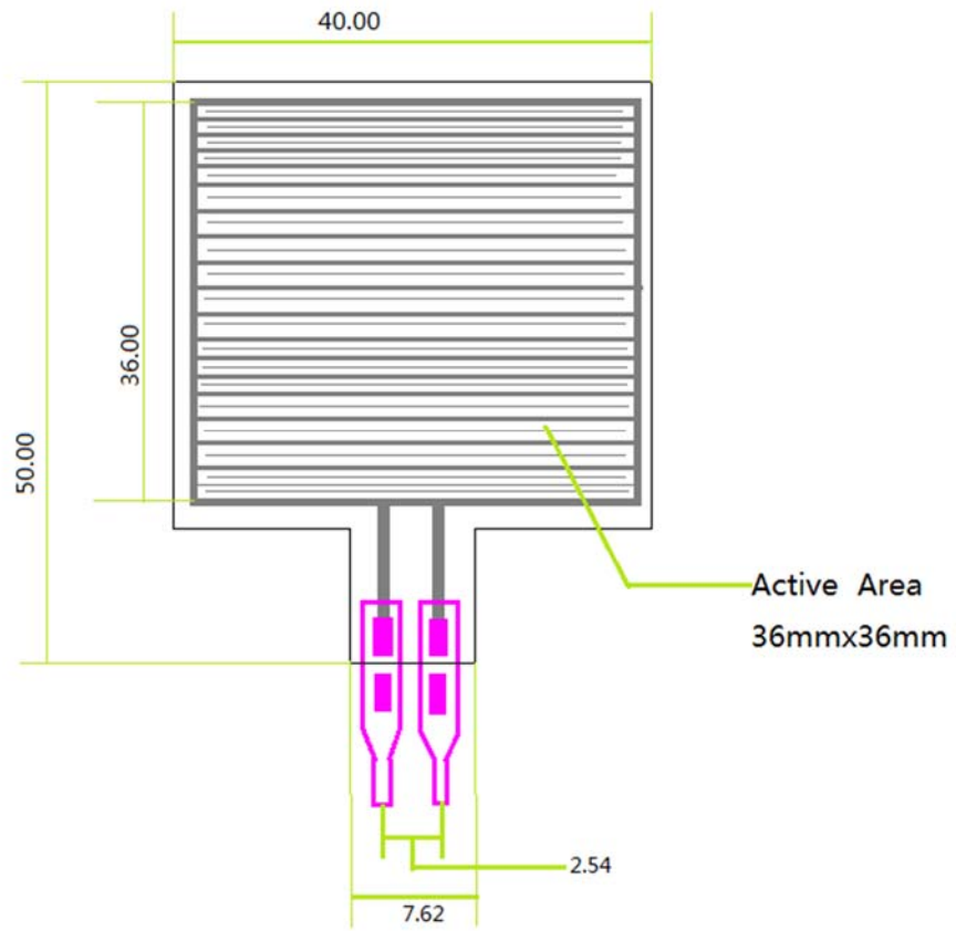
RP-S40-ST Dimension Diagram
