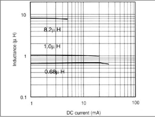
SDFL1005 Series Inductance vs. DC Current Characteristics
