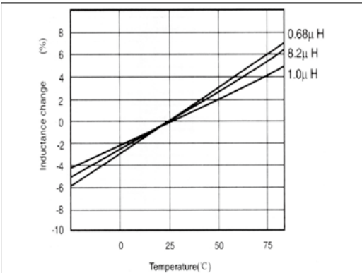
Inductance vs. Temperature Characteristics
