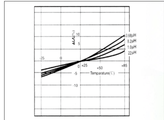
Inductance vs. Temperature Characteristics
