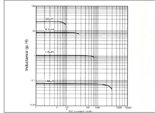
SDFL1608 Series Inductance vs. DC Current Characteristics
