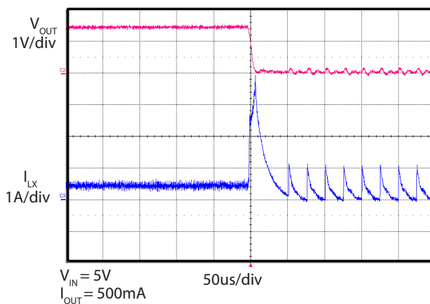
Output Hard Short ( V_{out}=1.5V )
