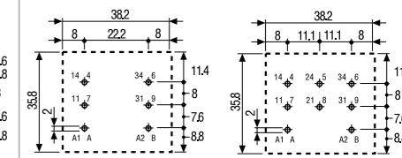
62.22 - 0300 Copper side view
