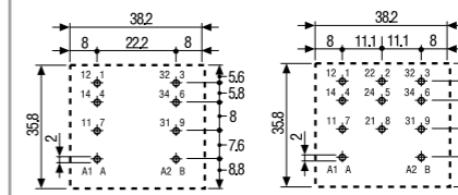
62.22 Copper side view
