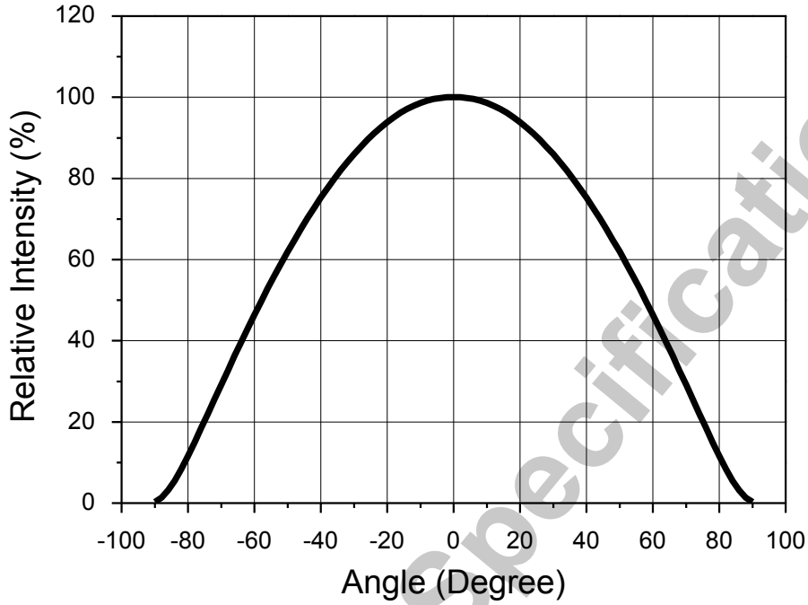
Fig 2. Radiant Pattern
