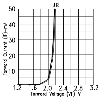
Fig3. FORWARD CURRENT VSE FORWARD VOLTAGE
