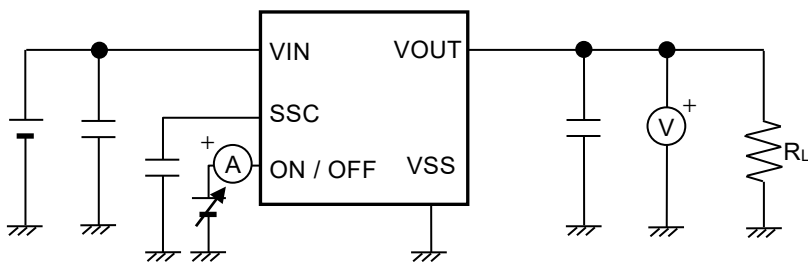
Figure 6 Test Circuit 4
