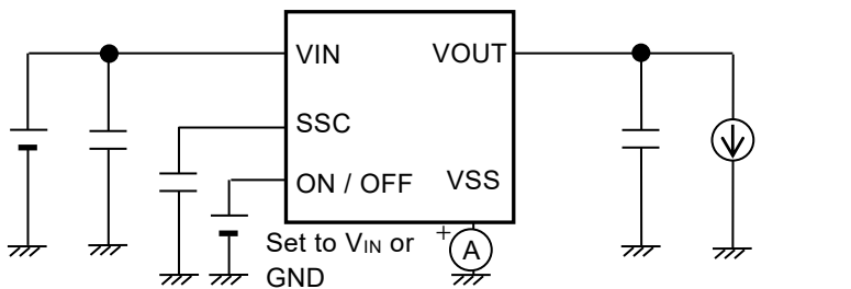
Figure 4 Test Circuit 2
