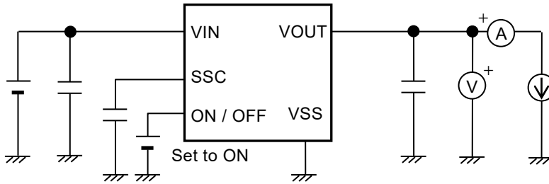
Figure 3 Test Circuit 1
