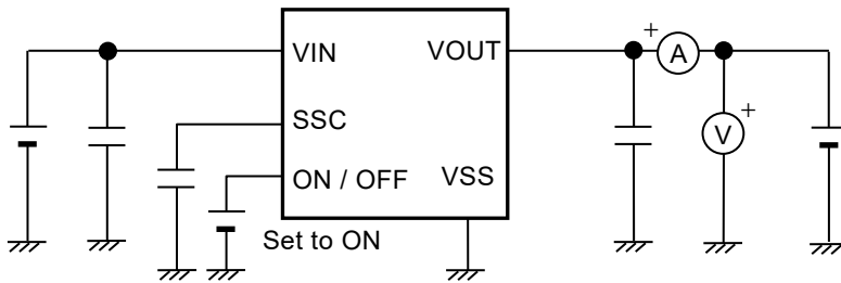
Figure 5 Test Circuit 3
