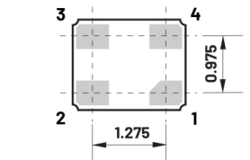
pads viewed from bottom pad size (0.72 x 0.55)mm
