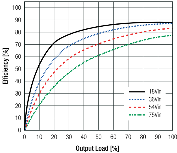
R1M-4812S/SMD Efficiency vs. Load
