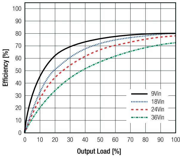
R1M-2405D/SMD Efficiency vs. Load
