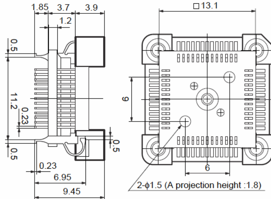
< Bottom view >
