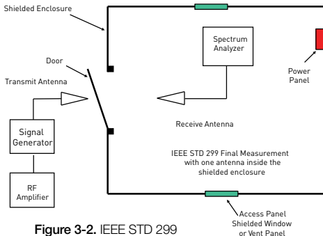
Figure 3-2. IEEE STD 299
