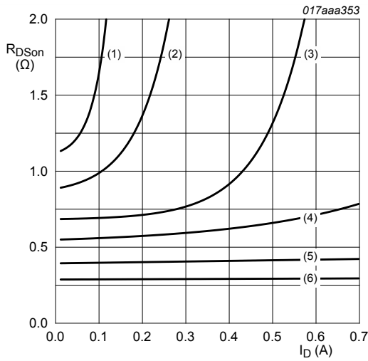
Fig. 8. Drain-source on-state resistance as a function of drain current; typical values (1) V_{GS} = 1.3 \text{ V} (2) V_{GS} = 1.4 \text{ V} (3) V_{GS} = 1.6 \text{ V} (4) V_{GS} = 1.8 \text{ V} (5) V_{GS} = 2.5 \text{ V} (6) V_{GS} = 4.5 \text{ V}
