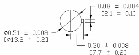
Mounting Hole
