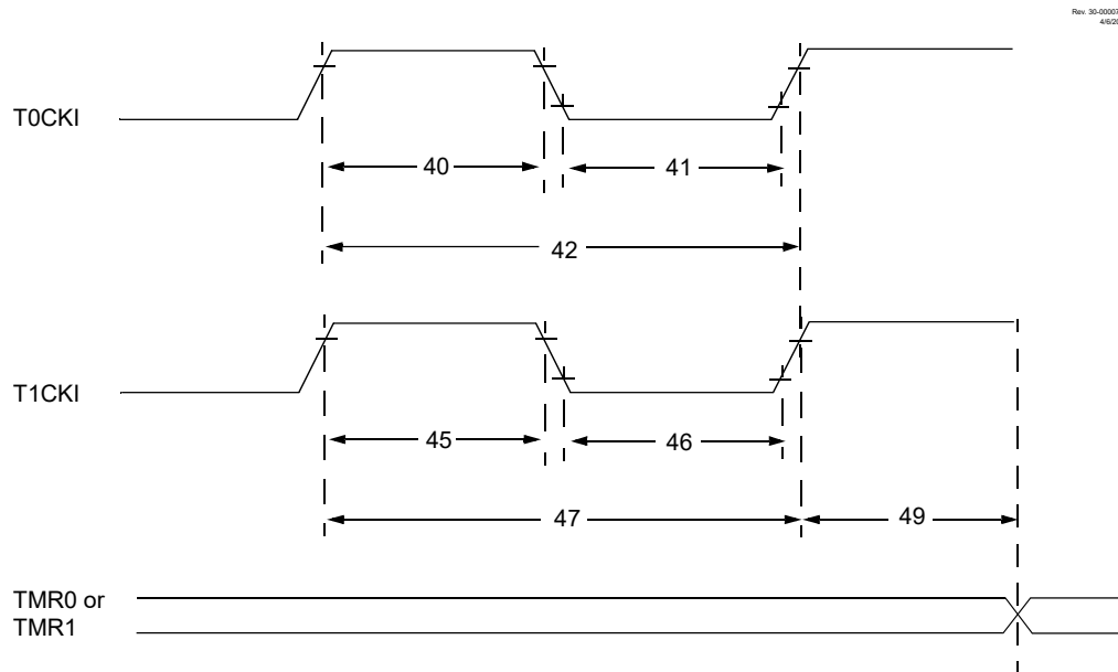
Figure 43-11. Timer0 and Timing1 External Clock Timings
