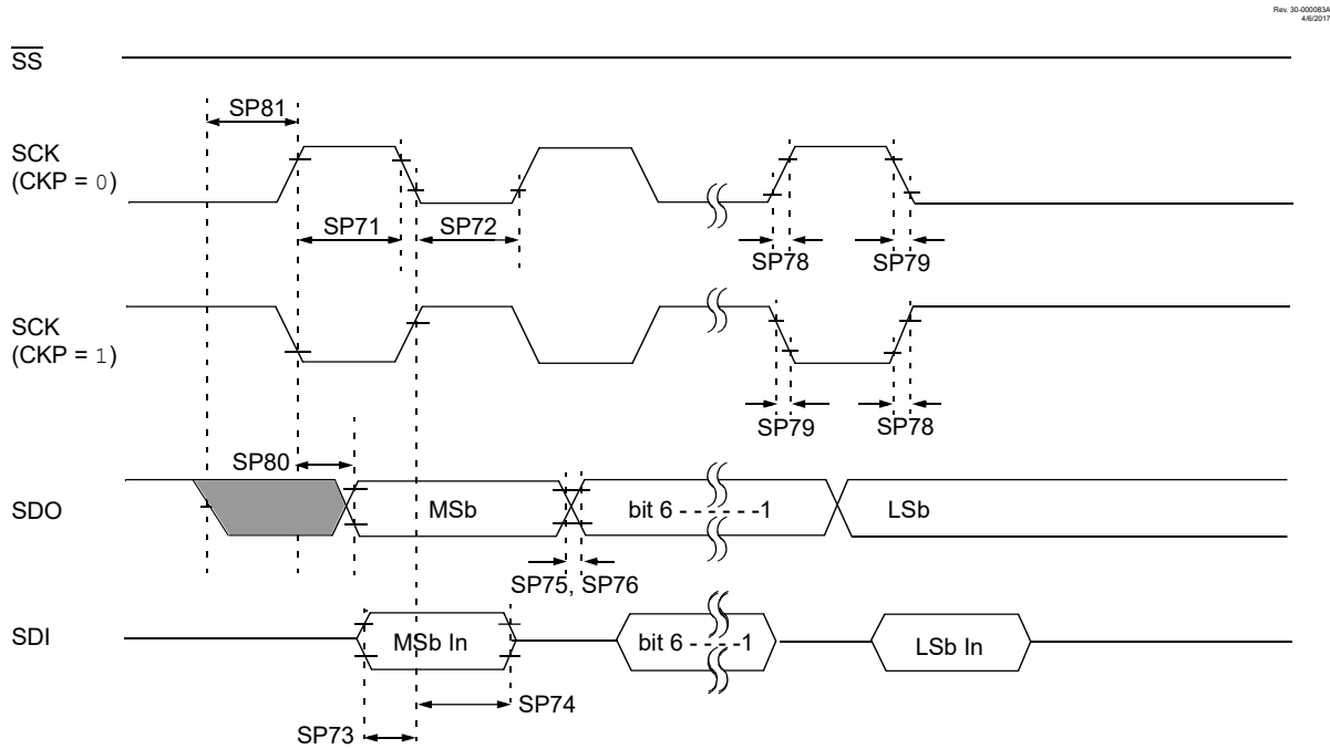
Figure 43-15. SPI Host Mode Timing (CKE = 0, SMP = 0)
