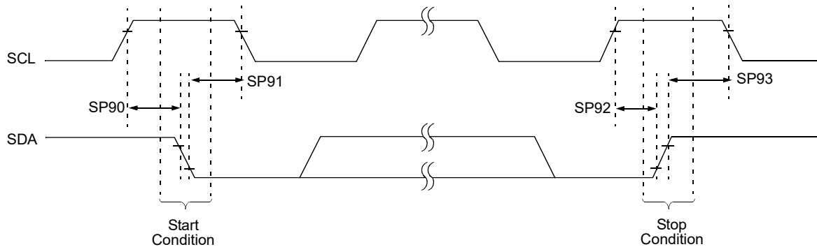
Figure 43-19. I 2 C Bus Start/Stop Bits Timing
