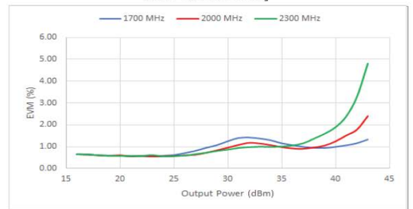
Error Vector Magnitude vs. Output Power [QPSK, 1Msps, 35% Roll Off Rate]
