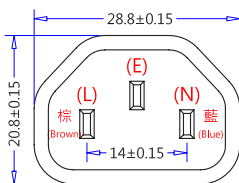
(IEC 60320, C14) (Dimensions of Plug Face)
