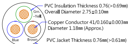
SJT 18AWGx3C (Wire Cross-Section)
