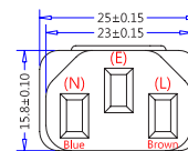
(IEC 60320, C13, 10A 250V~) (Dimensions of Connector Face)
