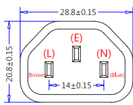
(IEC 60320, C14) (Dimensions of Plug Face)
